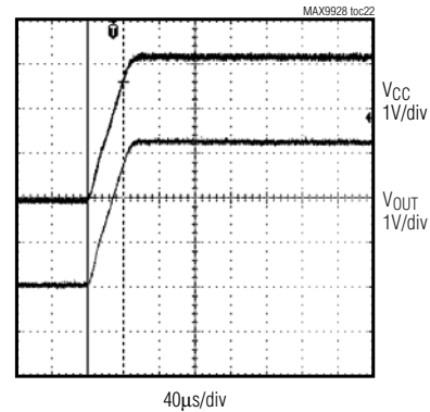
POWER-UP DELAY
